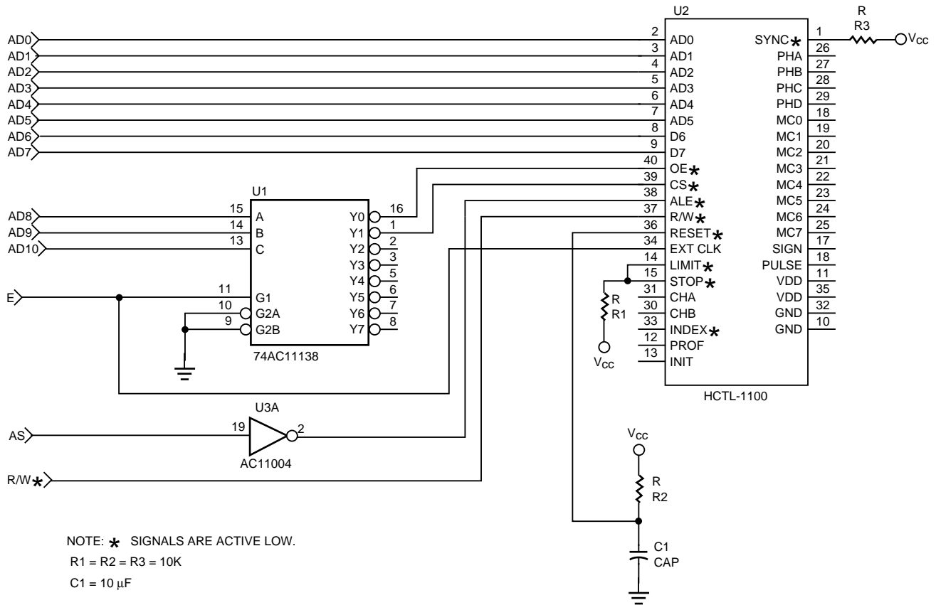
Figure 2. 68HC11 to HCTL-1100 Bus Interface.
