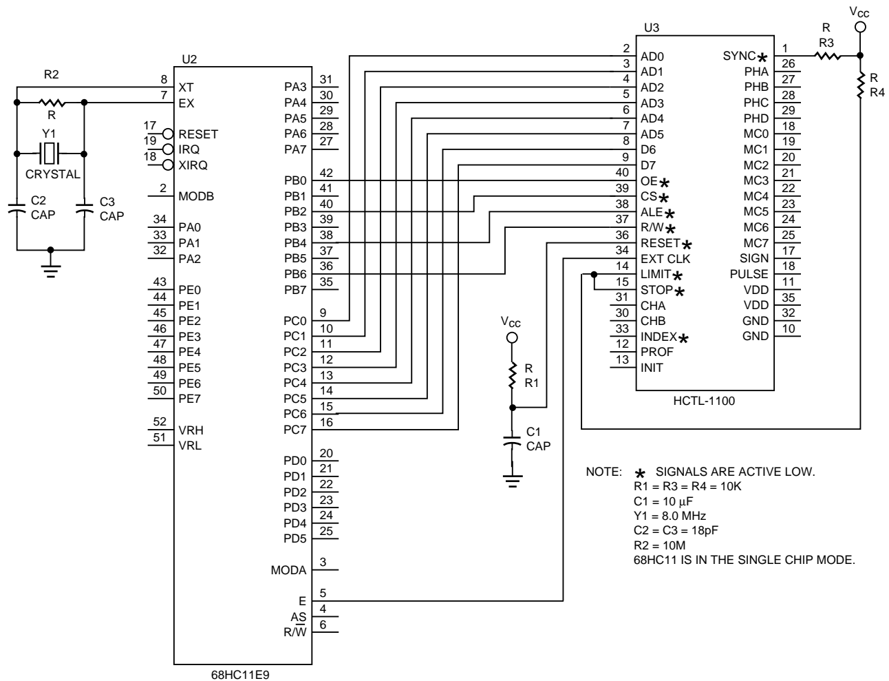
Figure 1. 68HC11 to HCTL-1100 Port Interface.
